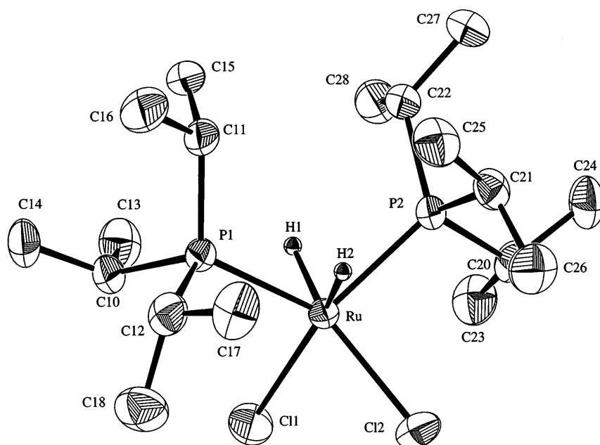
Figure 1. Molecular structure (ORTEP plot) of 4 ; [a] the hydrogen atoms besides H1 and H2 are omitted for clarity
