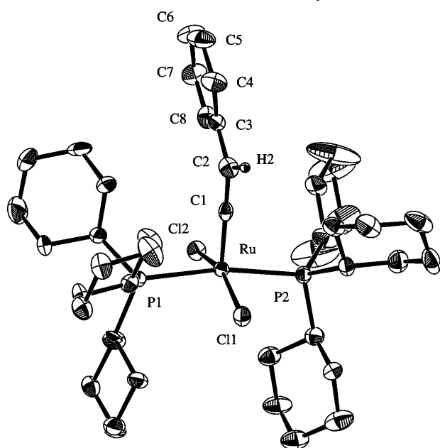
Figure 2. Molecular structure (ORTEP plot) of 15 ;[a] the hydrogen atoms are omitted for clarity
